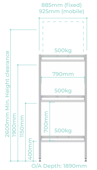
4H823BP / 4H823BPM (Mobile)
